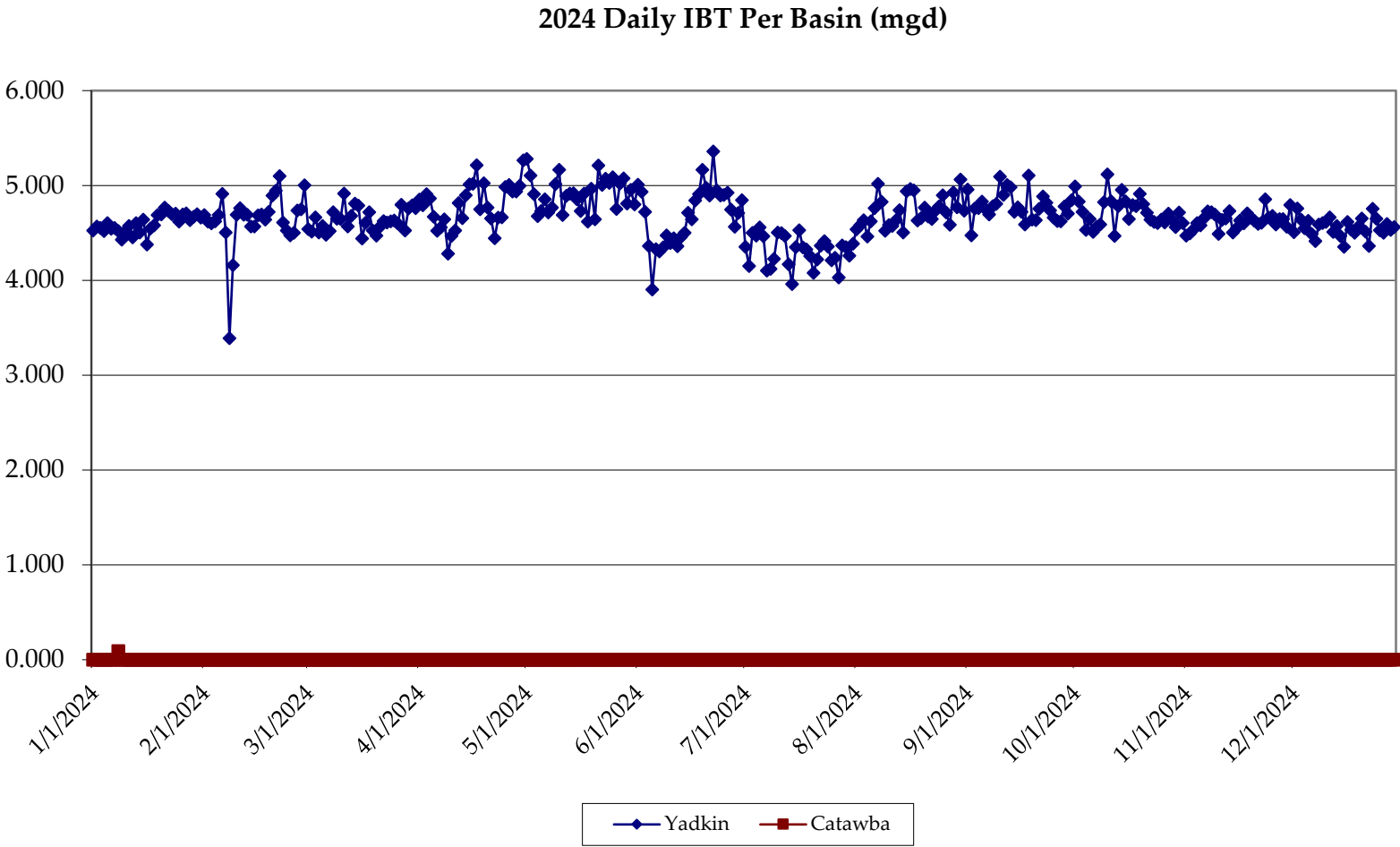
Figure ES-1 2024 Daily Interbasin Transfers by Basin
