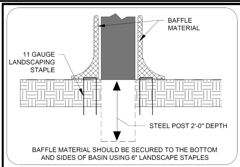
Figure 6.65b , Porous Baffle detail and cross section of a porous baffle in a sediment basin
