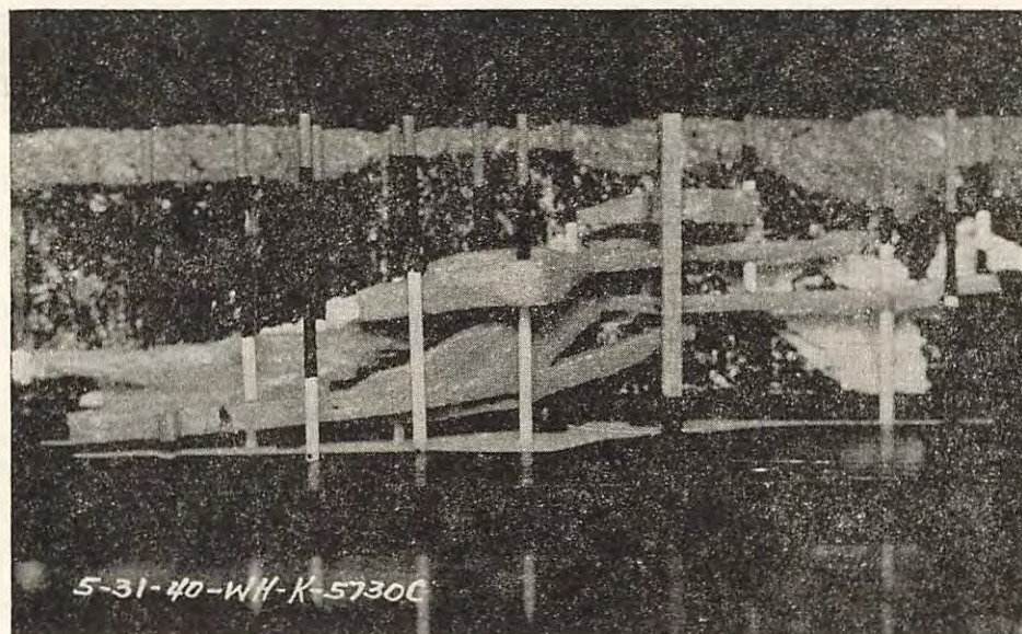
FIG. 7.—MODEL SHOWING UNDERGROUND WORKINGS AT THE CAROLINA TALC MINE. WHITE PARTS OF PEGS REPRESENT TALC ENCOUNTERED IN DRILL HOLES. LOOKING NORTHWEST.
