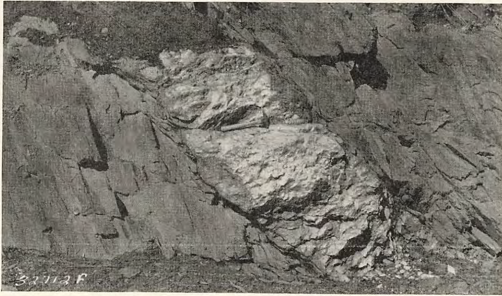
FIG. 1.—LARGE QUARTZ VEIN CUTTING QUARTZ-OTTRELITE GNEISS. RIGHT BANK OF THE HIWASSEE RIVER, OPPOSITE LOVER'S LEAP, NEAR MURPHY. LOOKING NORTHEAST.
