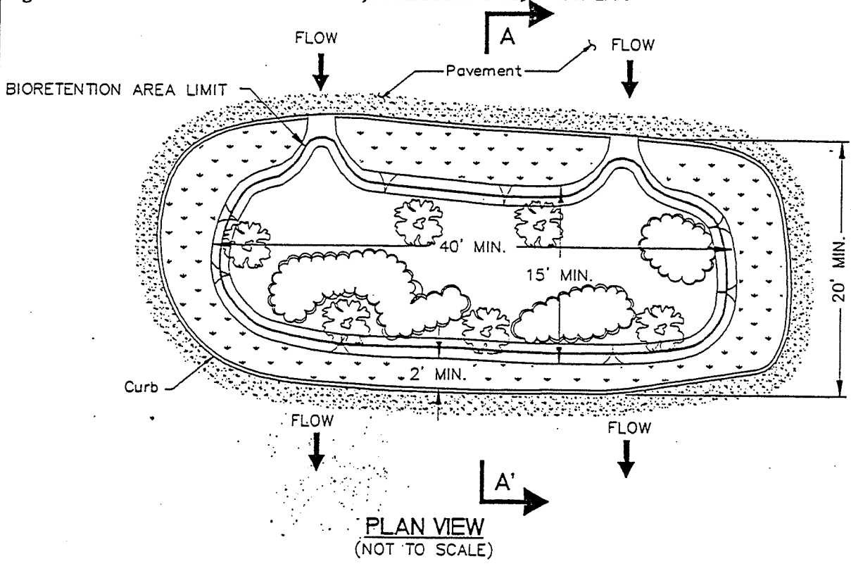
Figure 10. Traffic Island Bioretention Area, From Prince George's Co. 1993
