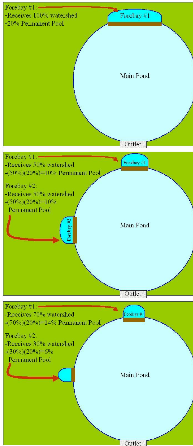
Figure 10-3c Forebay Sizing
