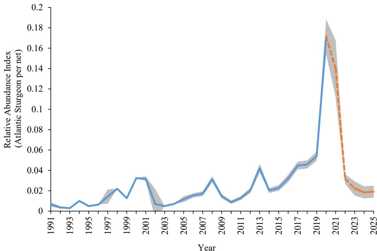
Figure 1. Annual nominal relative abundance index with SE shaded in gray for Atlantic Sturgeon collected from the Albemarle Sound Independent Gill Net Survey, 1991–2025. Note: survey methodology changed in November 2021 to reduce sturgeon interactions.
