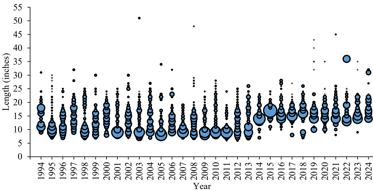
Figure 7. Recreational length frequency (total length, inches) of black drum harvested from 1994 to 2024. Bubbles represent fish at length and the bubble size is proportional to the number of fish at that length.
