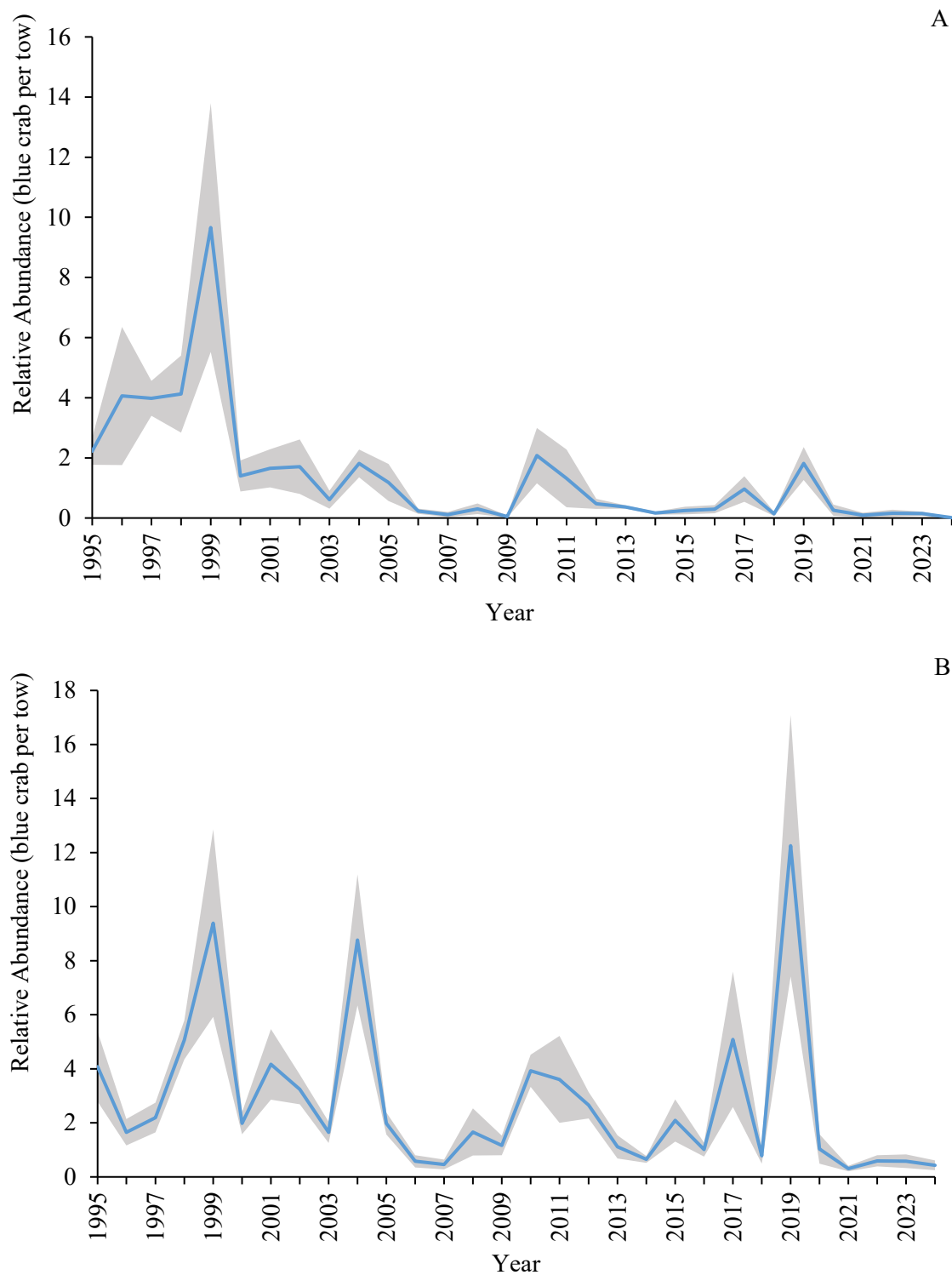
Figure 13. Nominal index (number of crabs per tow) of fully recruited crab relative abundance ( \geq 127 mm, 5 inches, CW) captured in Program 195 for June male (A) and female (B), 1995–2024 for all strata combined [Note: in 2020 and 2021 less than 54 stations were sampled in both months].
