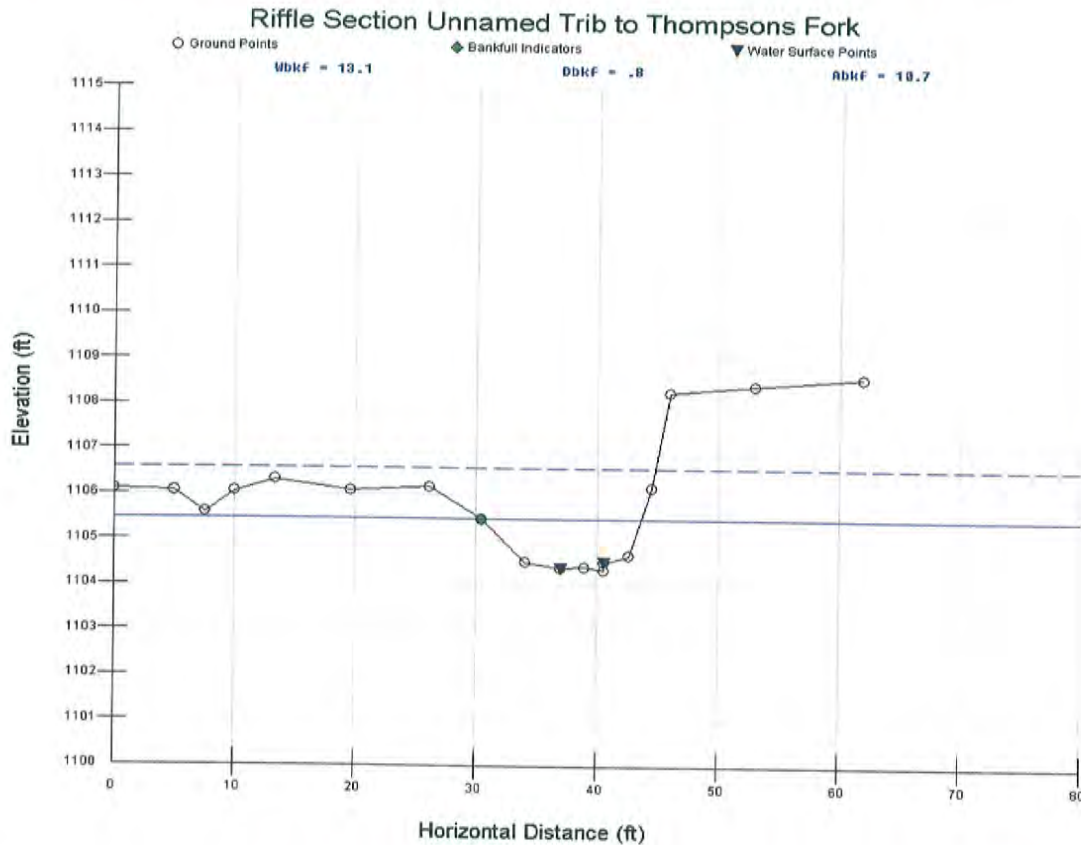
Thompsons Fork Unnamed Tributary Riffle Cross-Section, from left to right looking downstream.
