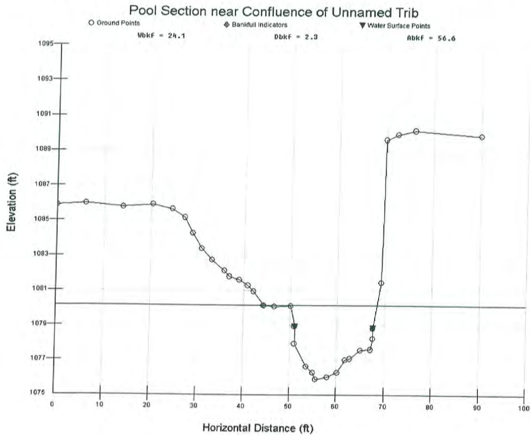
Thompsons Fork Mainstem Pool Cross-Section from left to right looking downstream.
