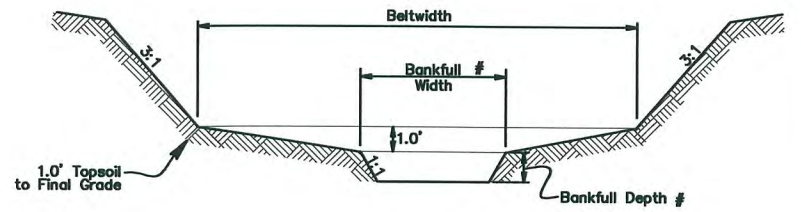
TYPICAL RIFFLE SECTION (See Detail 'B')
