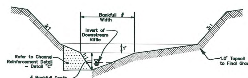
TYPICAL POOL SECTION (See Detail 'C')
