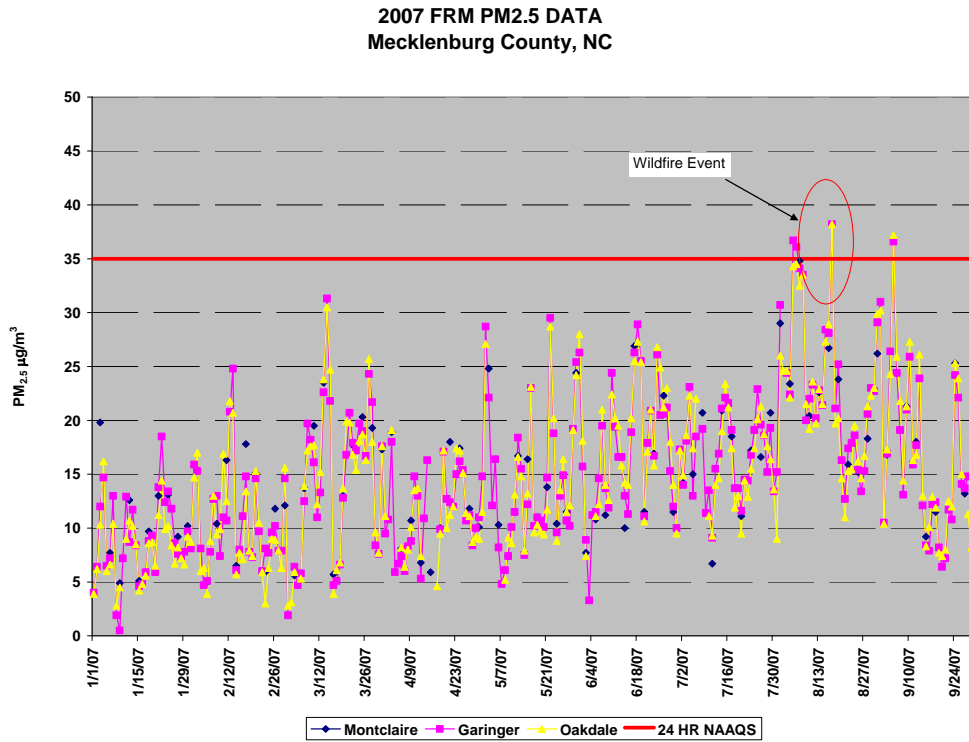
Figure 13. 2007 FRM PM 2.5 Data for Mecklenburg County
