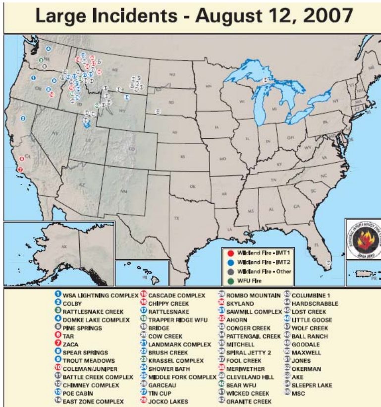
Figure 3 - Large fires – August 12, 2007
