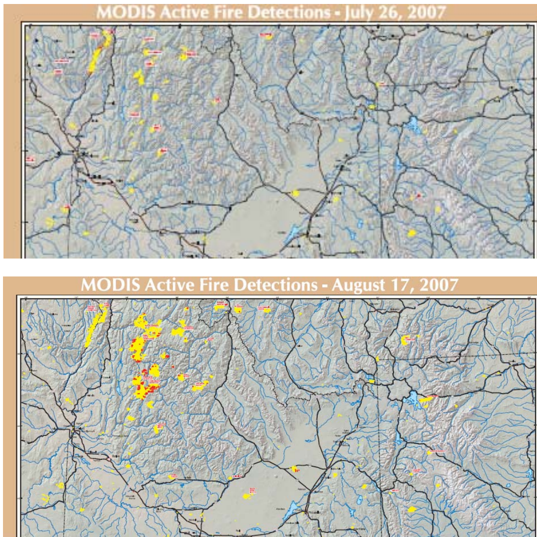
Figure 2. MODIS Active Fire Detection July 26, 2007 2 and August 17, 2007 Southern Idaho.
