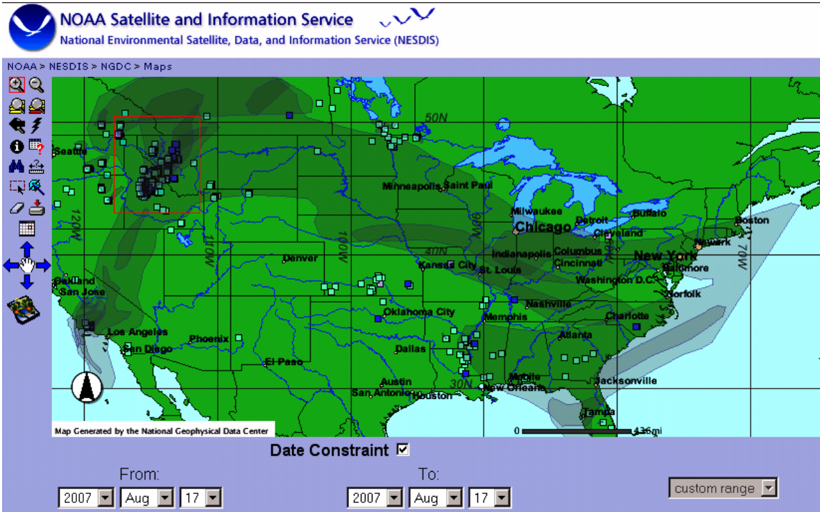
NOAA Satellite and Information Service, Analyzed Smoke – August 17, 2007 1 Figure 1.
