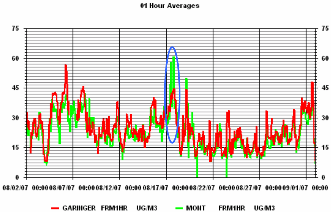
Figure 12. TEOM Data
