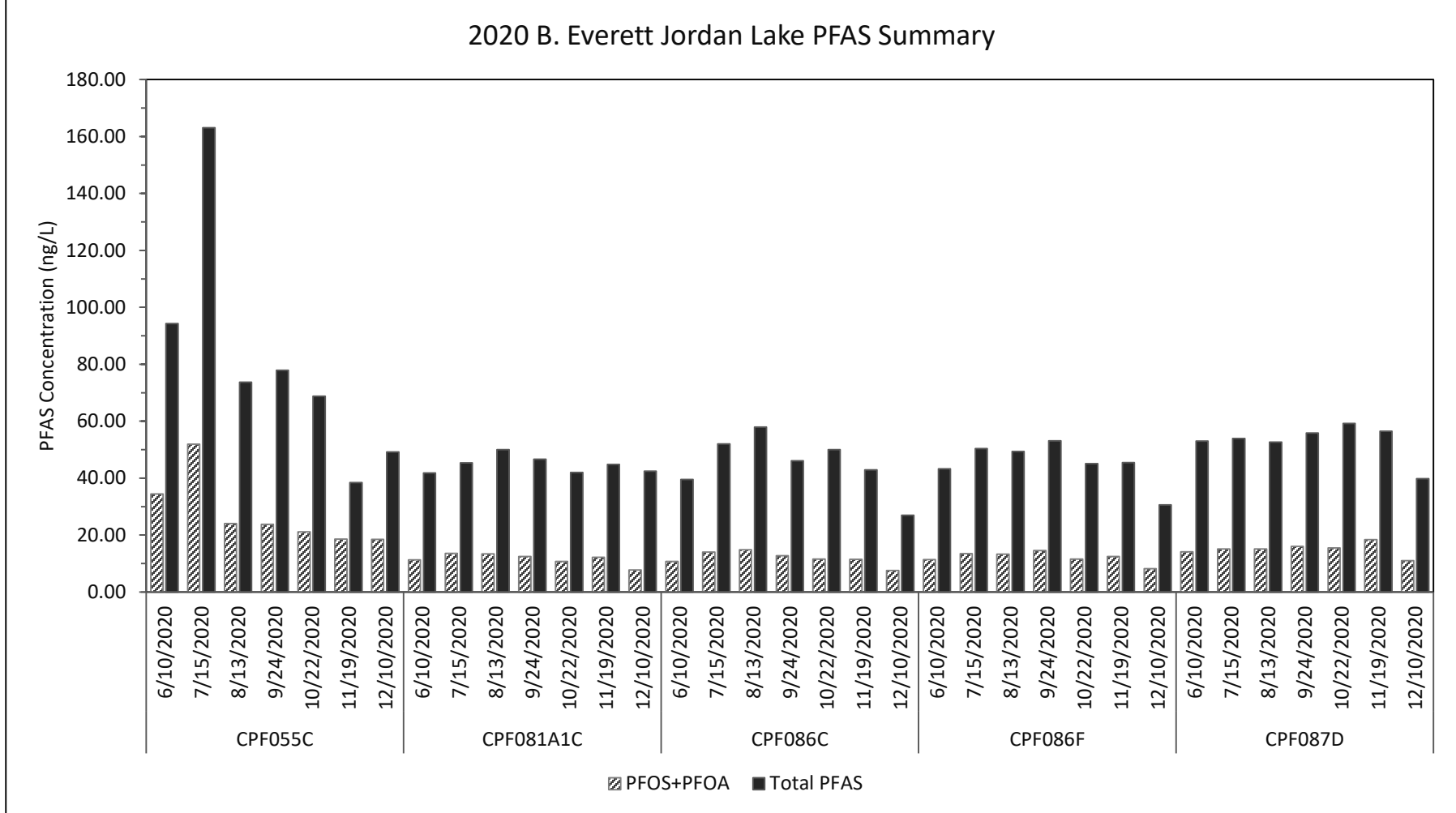
Figure 5. Per- and poly-fluorinated alkyl concentrations at B. Everett Jordan Lake monitoring stations. Only values greater than the PQL (2 ng/L) are presented.
