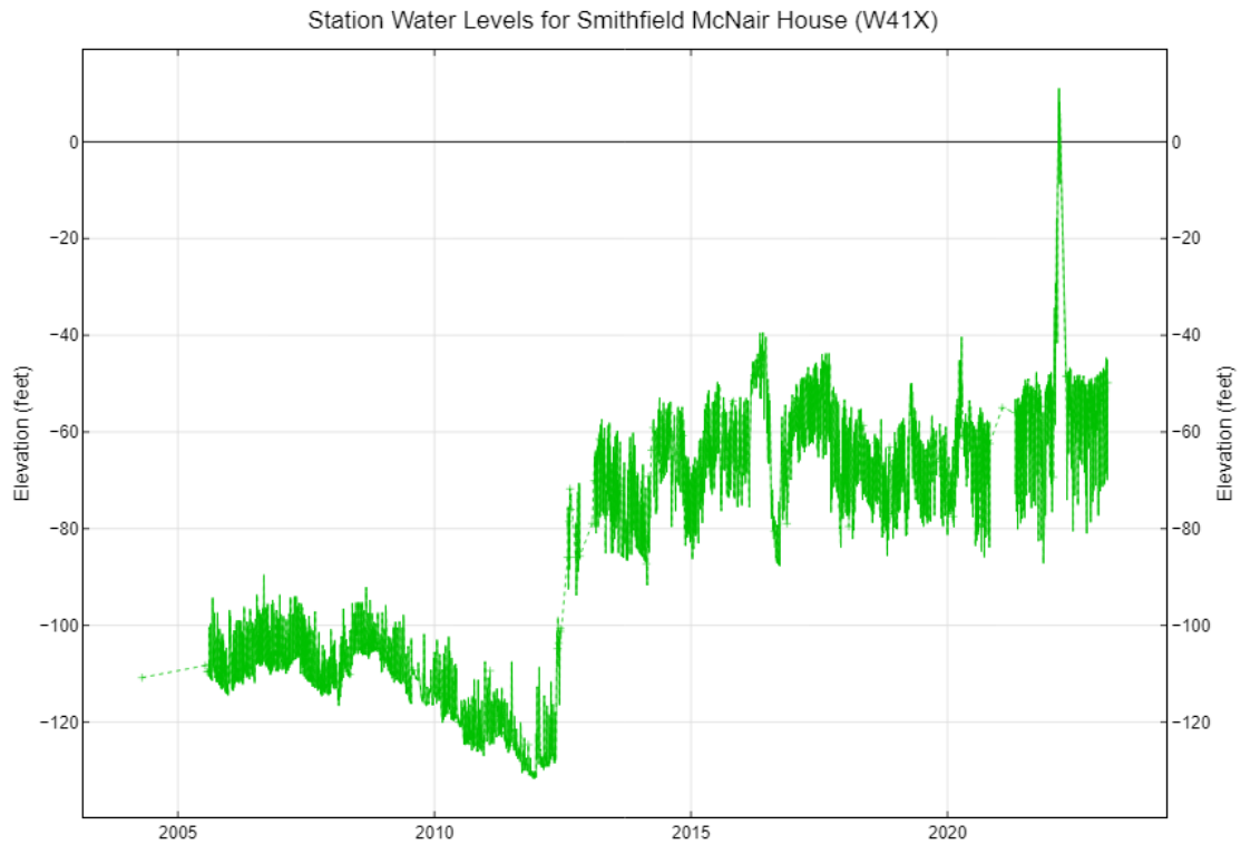
Figure 2 Water levels in groundwater monitoring well W41X for Smithfield McNair House.
