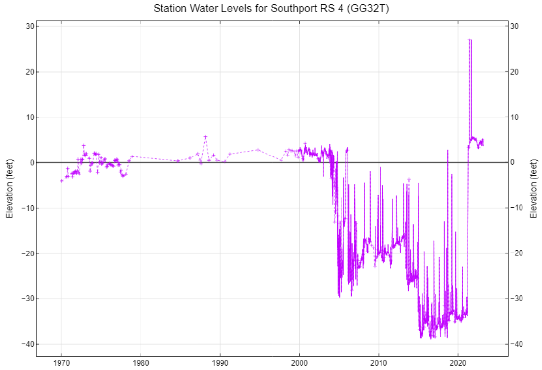
Figure 1 Water levels in groundwater monitoring well GG32T for Southport RS 4.
